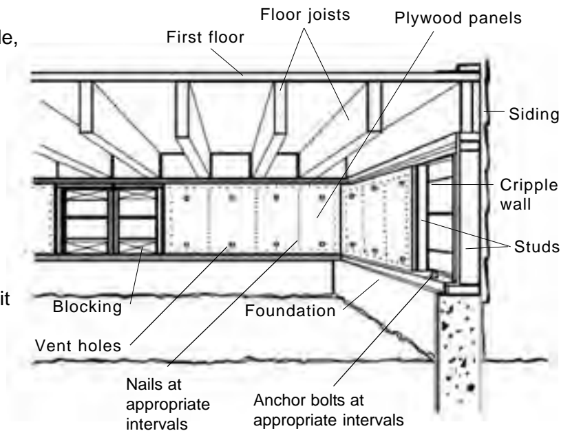
Figure 17—Plywood or diagonal sheathing strengthens weak cripple walls. If your home has a cripple wall between the foundation and the first floor, and the wall is not braced with plywood or diagonal sheathing, the house may fall or shift off its foundation during an earthquake.
