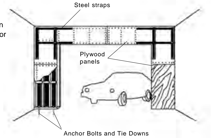
Figure 32—Bracing garage walls. If your house has a room over the garage, the garage walls may not be strong enough to hold up during an earthquake unless they are braced with plywood panels and steel straps.
